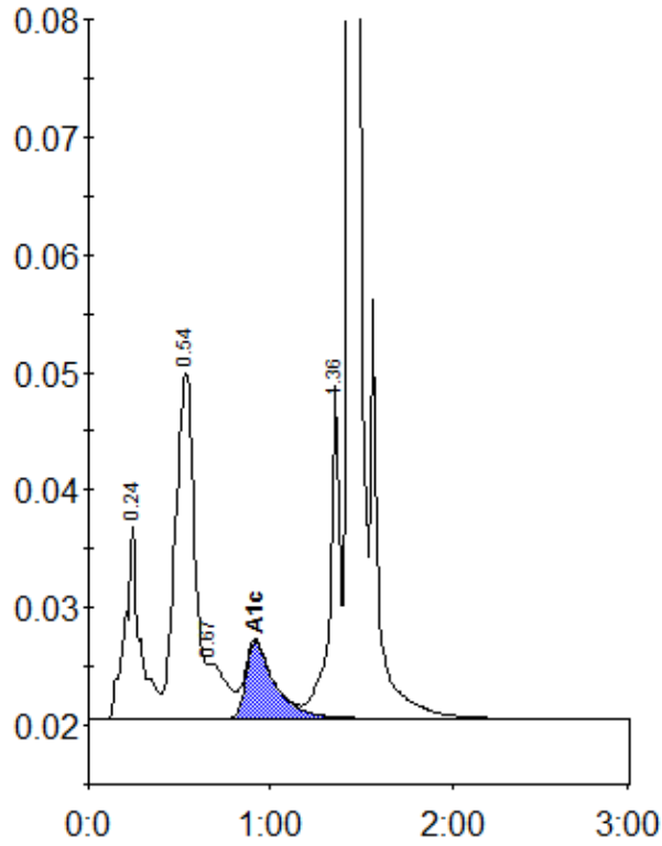
Peak table - ID: 10479574
